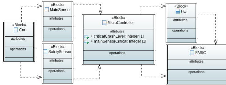
Fig. 3. bdd of the Airbag model
