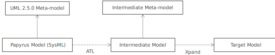
Fig. 2. Structure of the transformation
